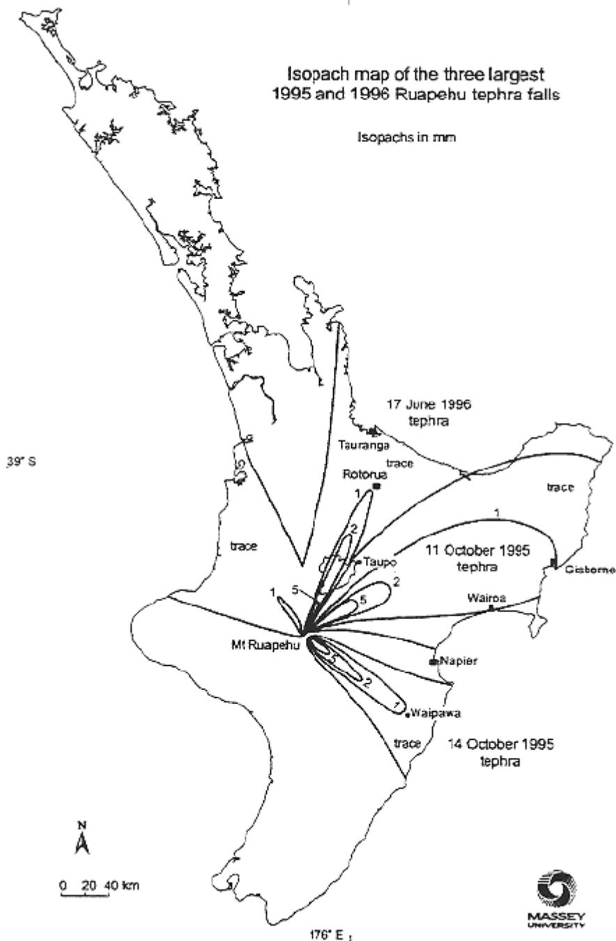
Figure 3.14: Isopach map of the three largest 1995 and 1996 Ruapehu tephra falls
