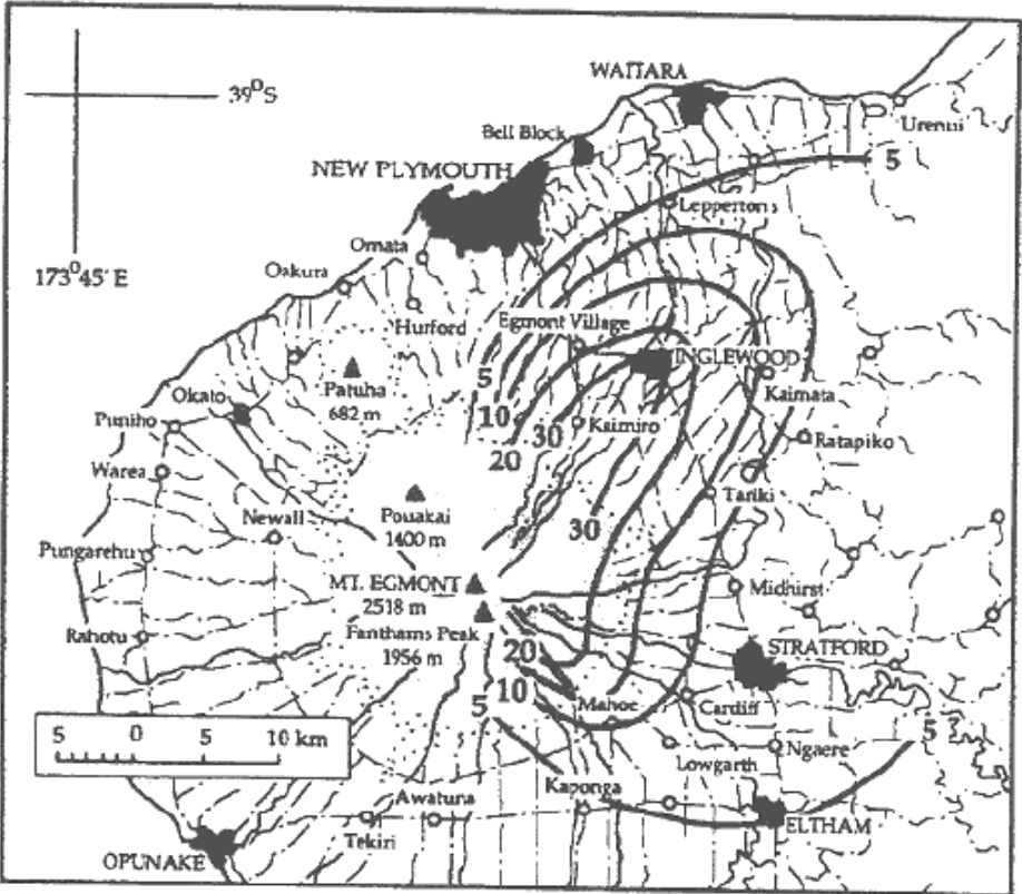
Figure 3.16: Isopach map (in centimetres) for the 3600 B.P. Inglewood Tephra. Map from Alloway et al 1995
