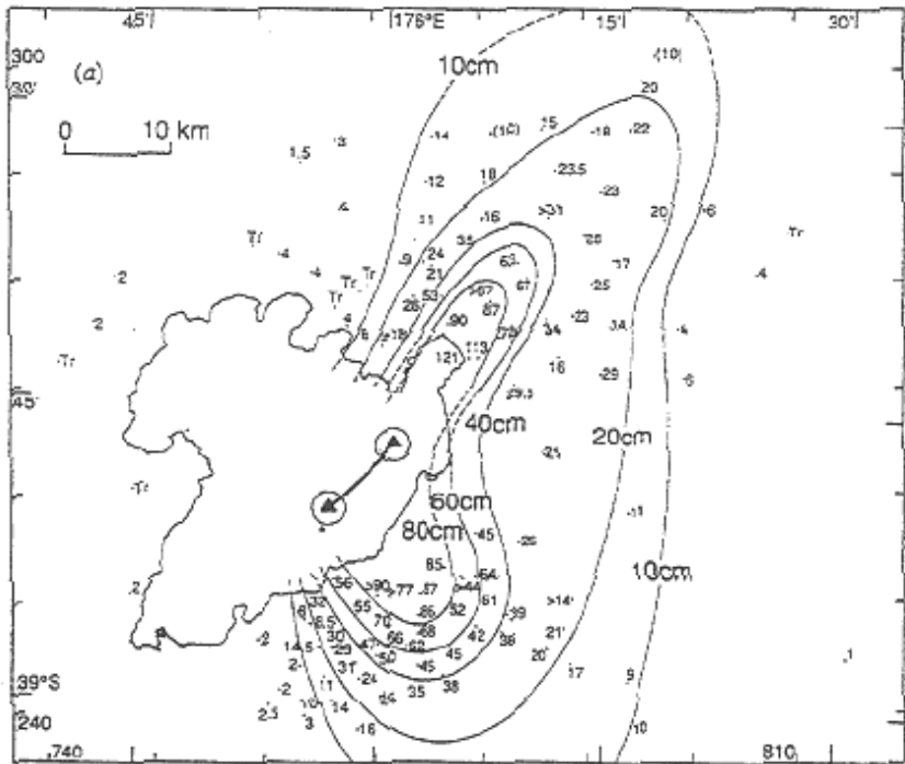
Figure 3.12: Isopach map of fall deposits erupted from multiple vents along a fissure with ends marked by filled triangles around 10 000 years B.P. Map from Wilson (1993)
