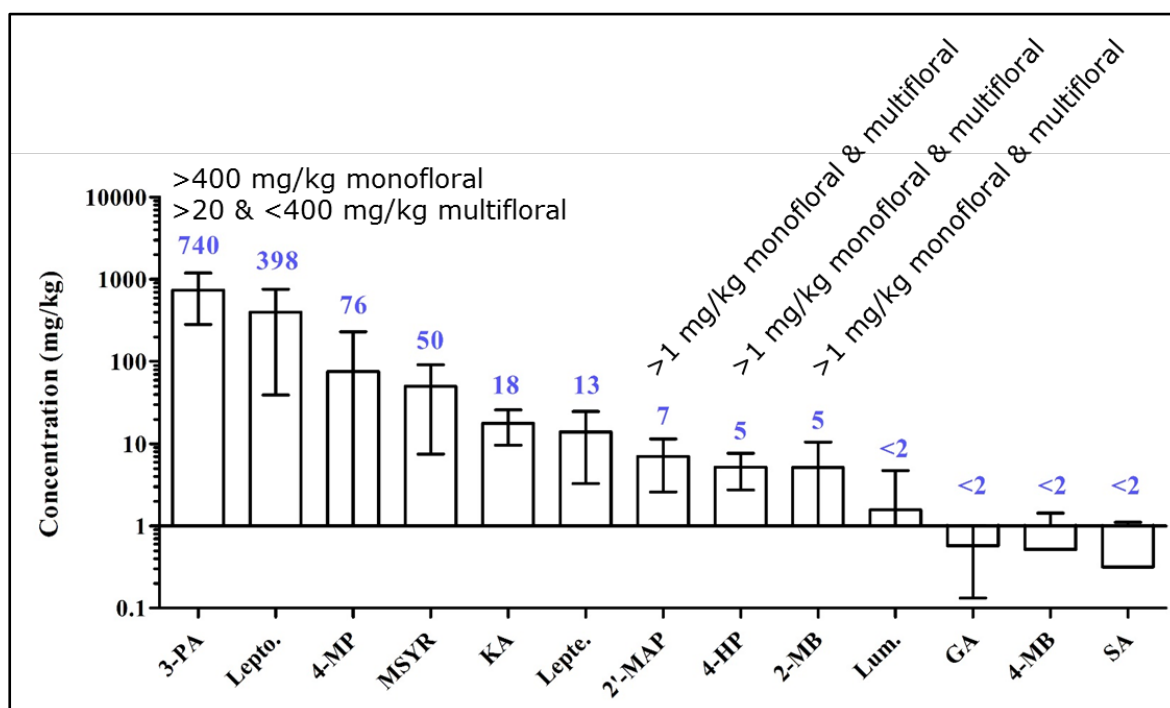
Figure 1. The mean concentration of 13 compounds present in manuka honeys. Error bars represent 1 SD.
