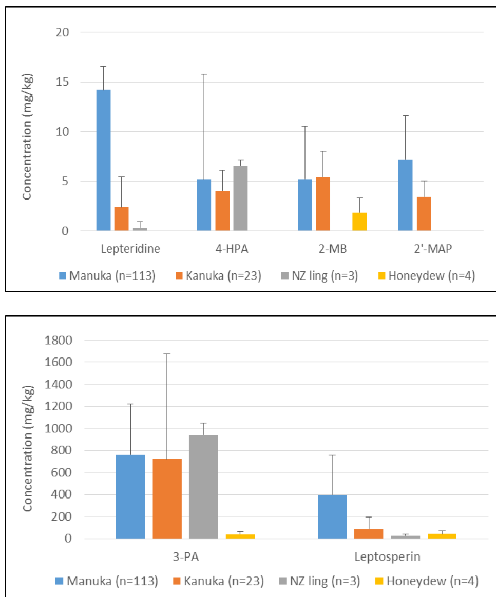
Figure 2. The mean concentration of 6 compounds present in manuka, kanuka, NZ ling, and honeydew honey. Error bars show 1 SD.
