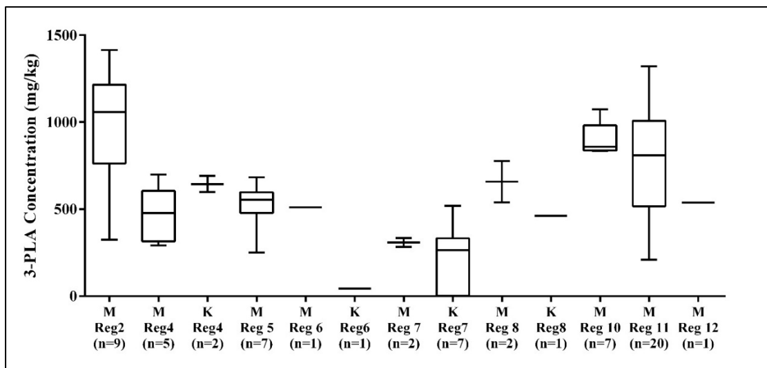
Figure 3. MPI honeys (2014/15 season). 3-PLA concentration for Manuka and kanuka honeys collected, some regions are not represented equally and some are missing.
