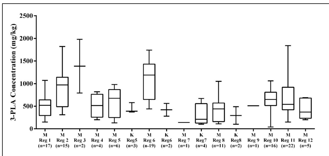
Figure 4. MPI honeys (2015/16 season). 3-PLA concentration for Manuka and kanuka honeys collected, some regions are not represented equally and some are missing.
