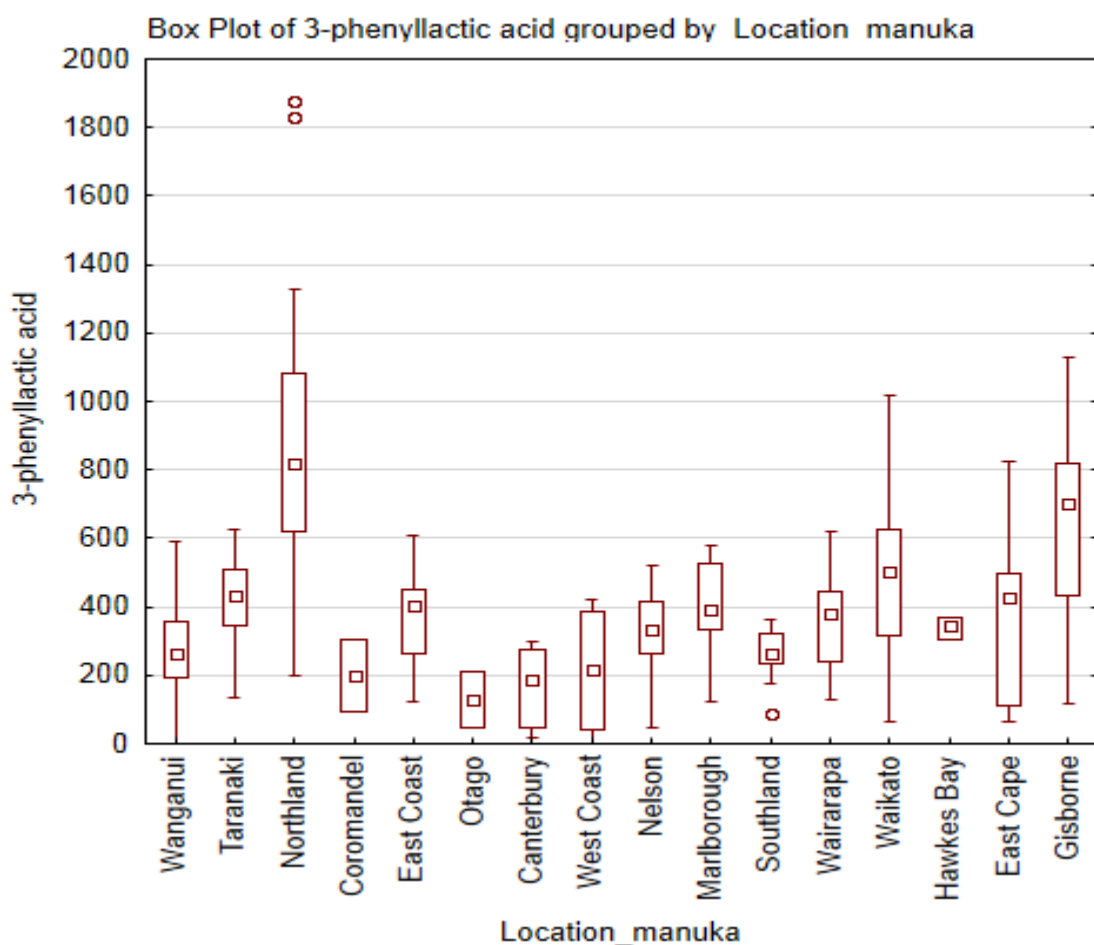
Figure 2. Variation in 3-PLA by region.
