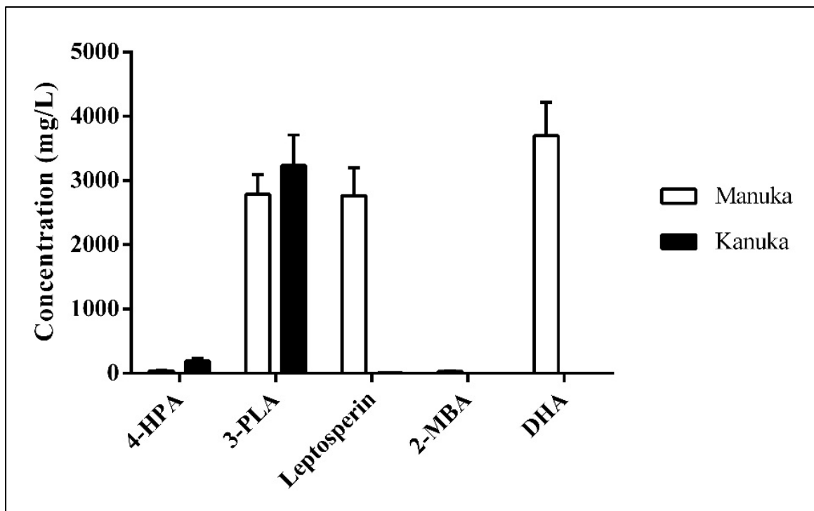
Figure 1. Nectar results from MPI data supplied to industry.
