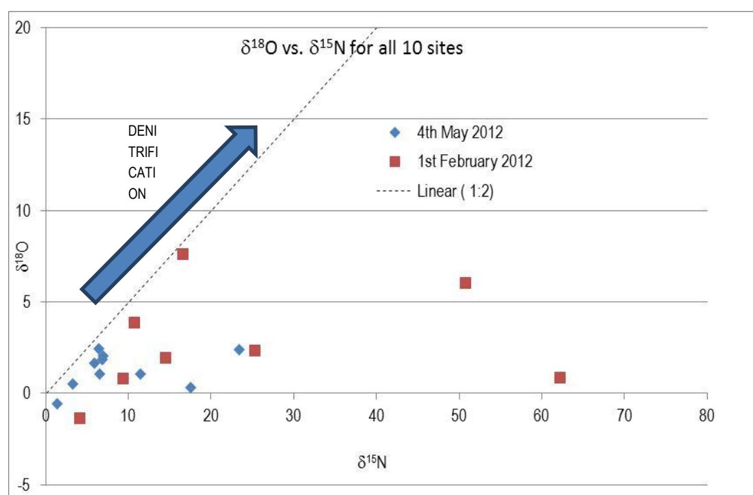
Figure 3.1: Plot of \delta^{18}\text{O} vs. \delta^{15}\text{N} for all ten sites on both sampling dates along with the linear 1:2 line.
