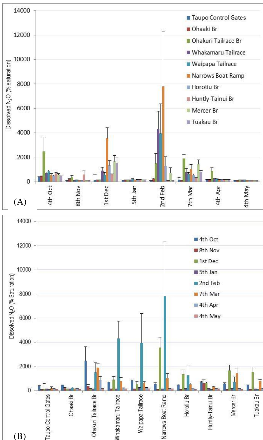
Figure 5.2: Average dissolved N_2O concentrations by sample date (A) and by site (B). Error bars are plus one s.e.m ( n = 3 ).
