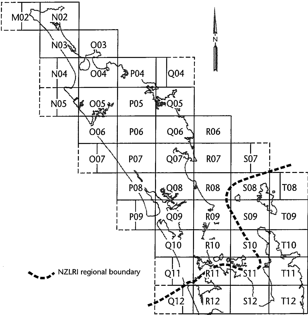
Figure 2. Location of the Northland region (NZLRI region 1), showing position of NZMS 260 map series.
