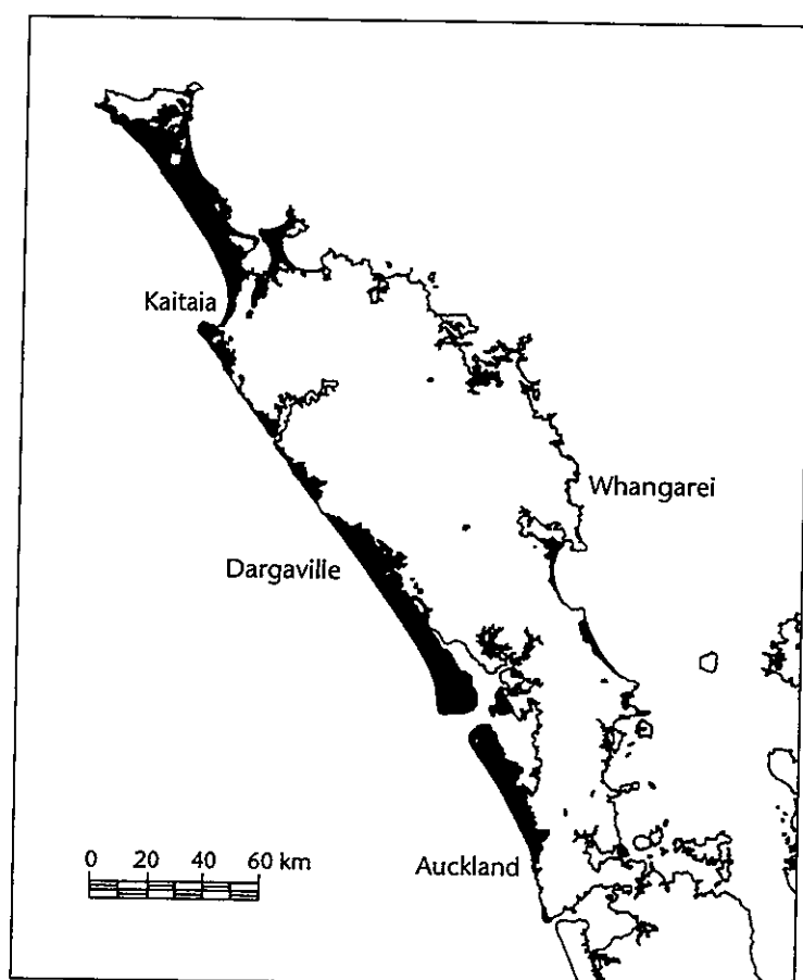
Figure 7. Location of LUC suite 1. Coastal sand country.
