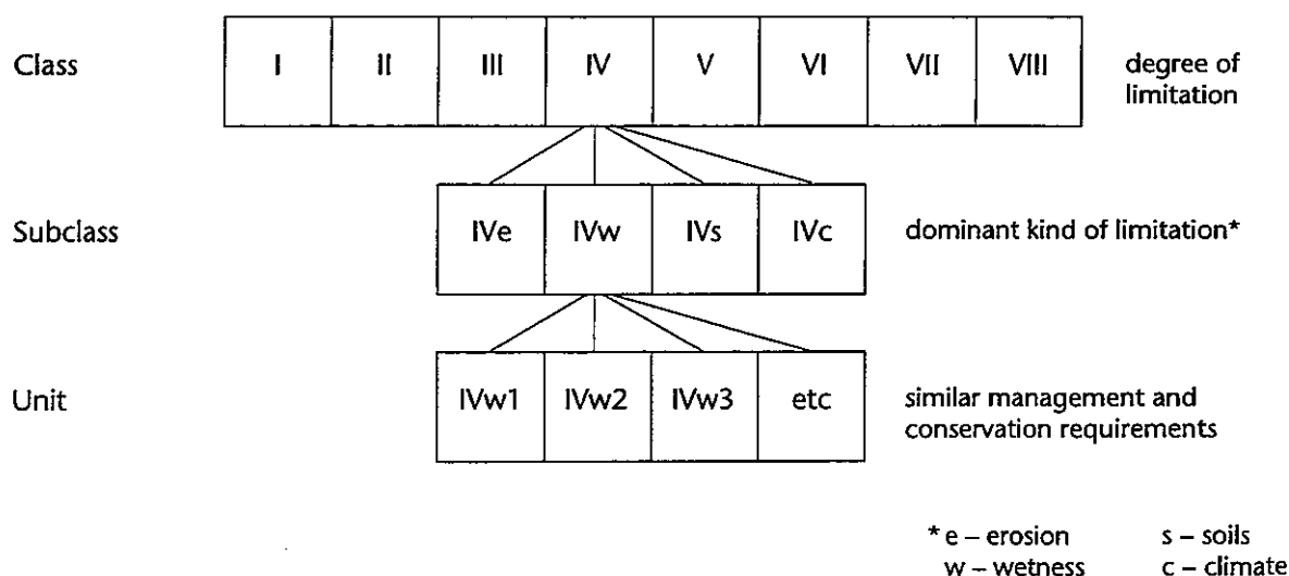
Figure 6. Components of LUC classification.
