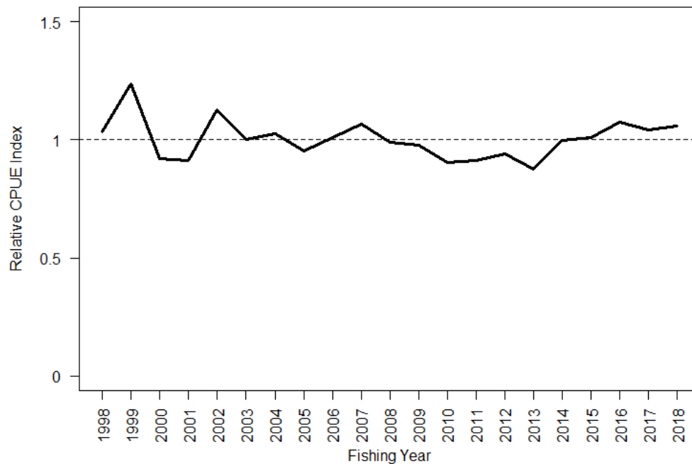
Figure 10: Standardised CPUE index for BCO 4 based on records of positive BCO catch by core vessels, 1997–98 to 2017–18 (Large et al in prep.).
