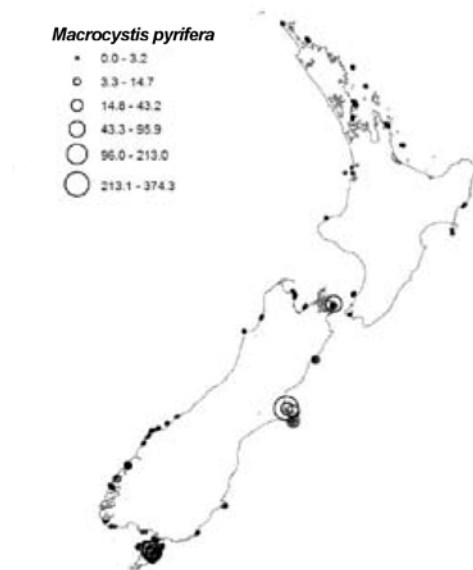
Figure 3: Mean biomass (g ash free dry weight m^{-2} ) of attached bladder kelp at all sites, averaged across 4 depth
