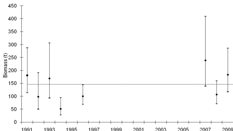
Figure 2: Biomass estimates \pm 95\% CI (estimated from survey CV's assuming a lognormal distribution) and the time series mean (dotted line) from the East Coast South Island trawl survey.
