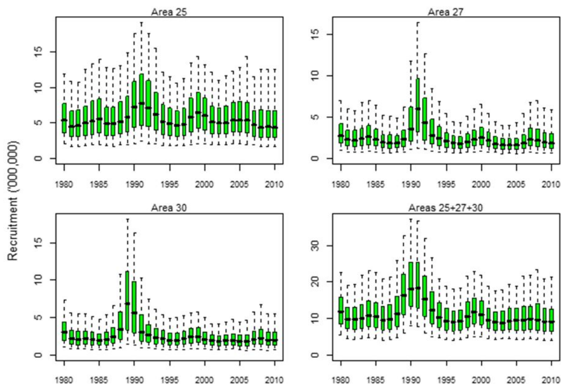
Figure 13: Recruitment estimates from the base case runs for Areas 025, 027, 030, and the Areas combined, 1980–2010. The boxes show the interquartile range, the whiskers show the 90% confidence limits, and the bars show the medians.
