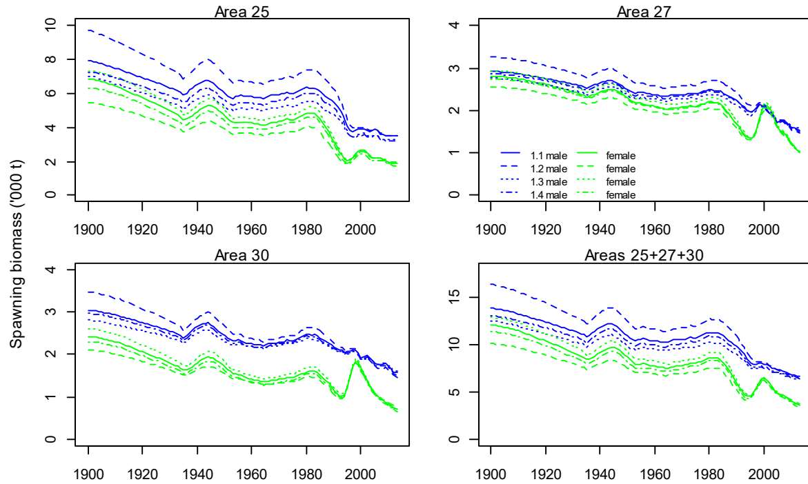
Figure 11: Median estimates of Area 025, Area 027, Area 030, and Areas combined male and female spawning biomass for the base case and sensitivity runs, 1900 – 2012.
