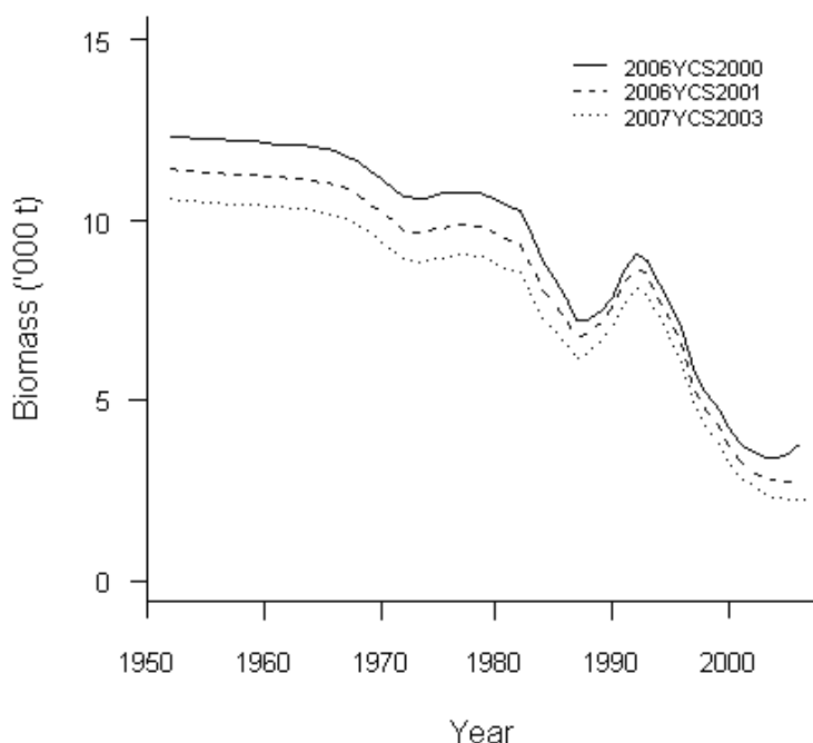
Figure 5: MPD biomass trajectories for the northern stock (SKI 1 & 2) from three model runs: 2006 YCS2000 , 2006 YCS2001 , and 2007 YCS2003 .
