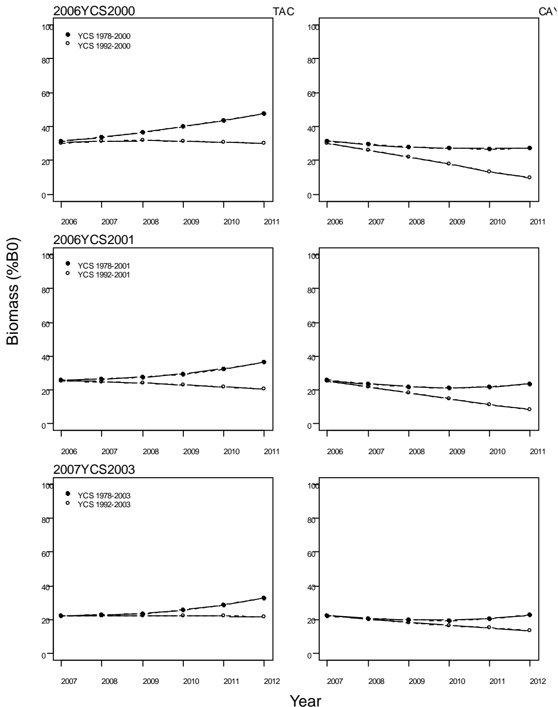
Figure 7: Bayesian median of projected biomass (% B_0 ) for the northern stock (SKI 1 and SKI 2) from three model runs, with future catch fixed at TAC or estimated CAY, and future recruitment randomly resampled from the long period or the recent period.
