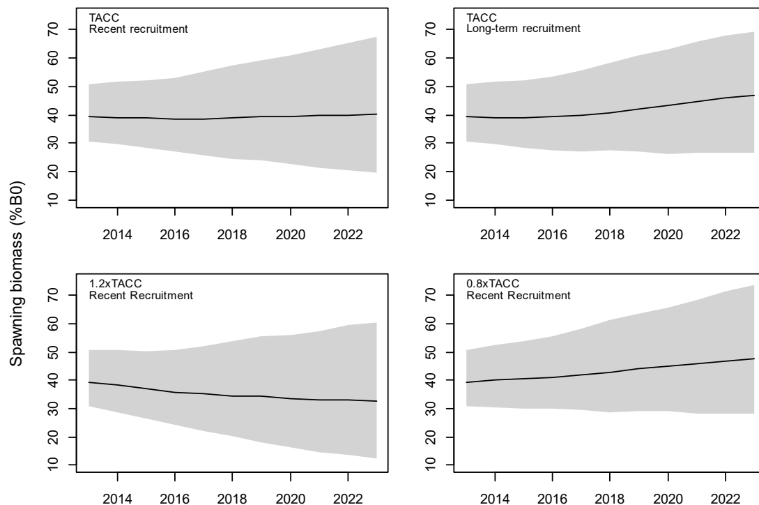
Figure 14: Projected BCO 5 spawning biomass (% B_0 ) assuming recent or long-term recruitment and catch at current TACC or increased/decreased by 20% for the base case run. Median estimates are shown as solid lines and 90% confidence intervals as shaded polygons.
