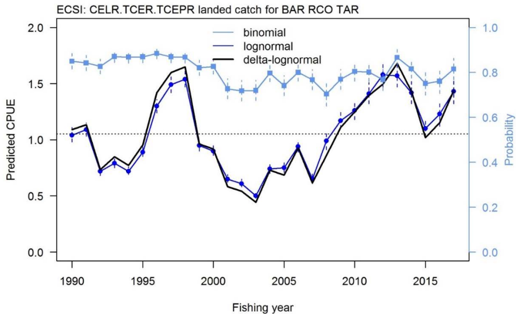
Figure 5 : East coast South Island part of BAR 1 CPUE indices from the standardised lognormal, binomial, and the combined (delta lognormal) models, based on the merged day-level CELR, TCER, and small vessel (<28m) TCEPR data for 1989–90 to 2016–17.
