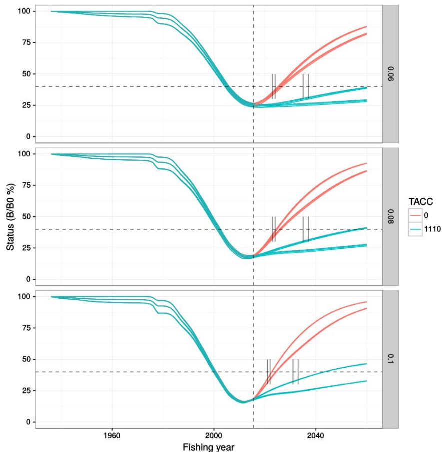
Figure 9: Projected SSB at different catch levels from the 2016 run with alternative levels of M and h and catch histories. The short vertical lines around 40% B_0 mark 2011 + T_{min} and 2011 + 2 T_{min} .
