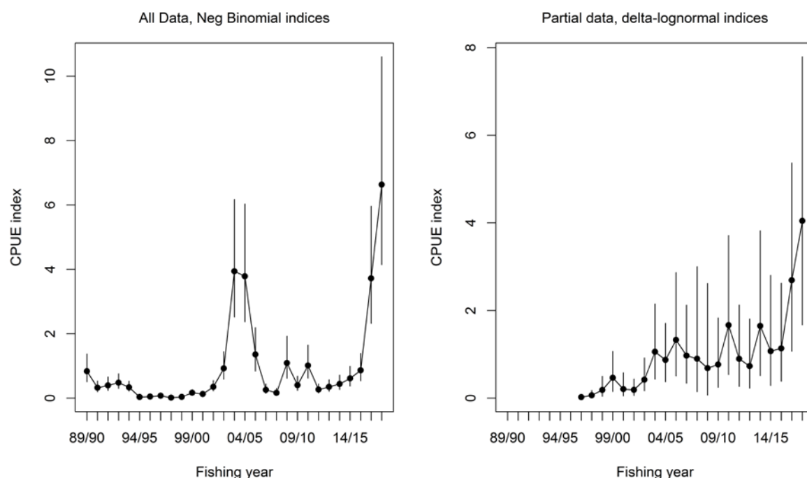
Figure 8: Gemfish (SKI 7) CPUE indices derived from the entire WCSI hoki fleet ( all data CPUE , left) and a subset of the fleet ( partial data CPUE , right). (Approximate 95% confidence intervals).
