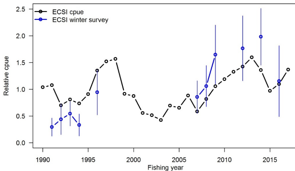
Figure 6: Comparison of the BAR 1 ECSI delta-lognormal CPUE series for 1990–2017 and the recruited biomass (and associated variance) from the ECSI winter trawl survey series. The recruited biomass is based on fish over 60 cm fork length. Each series has been standardised to the mean for concurrent years.
