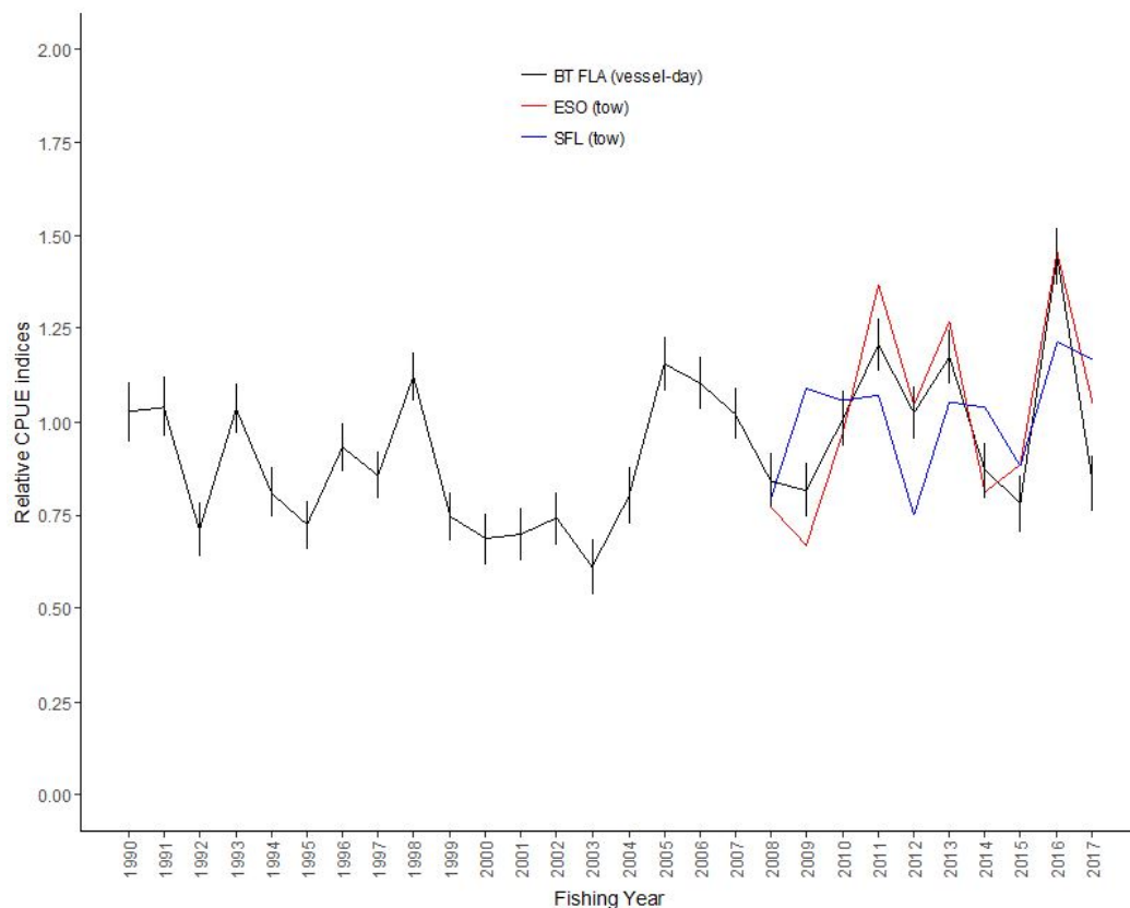
Figure 3: Standardised CPUE indices in FLA 2 for BT targeting all species of flatfish, (aggregated to combine data across form types, BT_flats(day)), and shorter combined series for sand flounder (BT_sfl(tow)) and New Zealand sole (BT_eso(tow)) based on tow by tow resolution data (Schofield et al 2018b).
