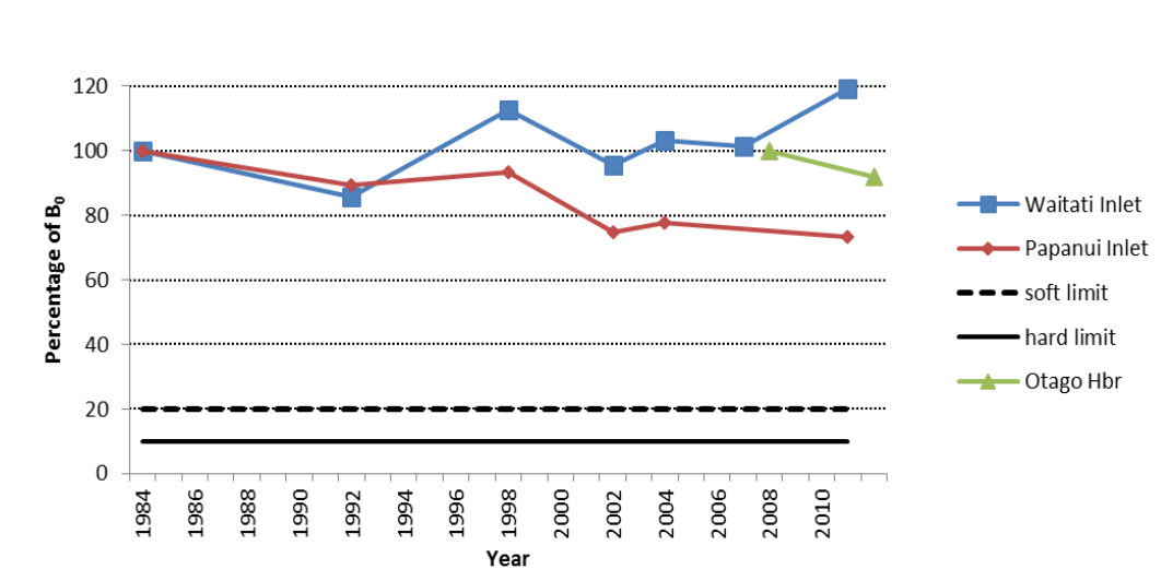
Figure 3: Biomass as a proportion of B_0 for Waitati and Papanui Inlets, this is estimated from biomass >19mm. Note: No catch has been taken from Papanui Inlet since 2006–07. Virgin biomass was taken from the Stewart 2008b survey for Otago harbour as this is the extent that has been subsequently surveyed.
