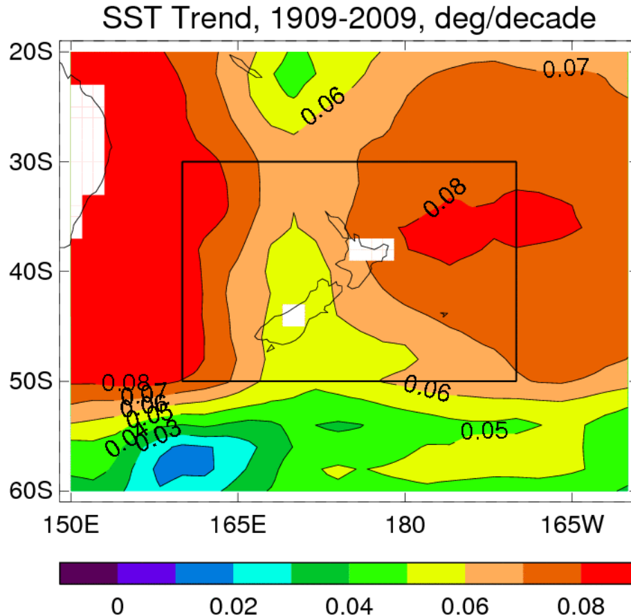
Figure 8.7: Trends in sea surface temperature, in °C/decade over the period 1909-2009, calculated from the NOAA_ERSST_v3 data-set (provided by NOAA's ESRL Physical Sciences Division, Boulder, Colorado, USA, from their web site at http://www.esrl.noaa.gov/psd/ ). The data values are on a 2° latitude-longitude grid. The box around New Zealand denotes the region used to produce the area-averaged sea temperatures plotted in Figure 2. (Image Source Mullan et al. 2010.)
