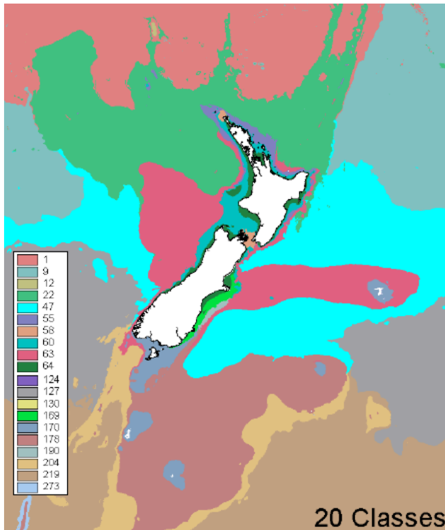
Figure 7.5: The 20-class version of the 2005 general purpose Marine Environment Classification (MEC, from Snelder et al. 2005). The class numbers are nominal; for attributes of each class at this level, see Table 7.1.
