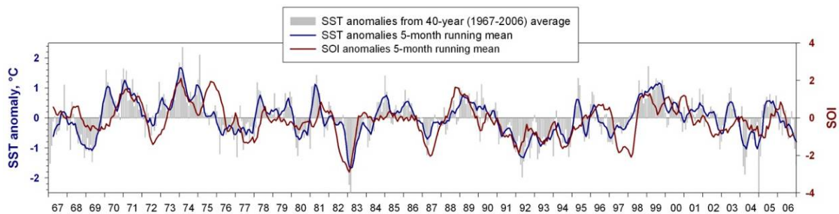
Figure 8.9: Sea surface temperature (SST) anomalies from SST measurements at Leigh (Auckland University Marine Laboratory) and Southern Oscillation Index (SOI) anomalies. (Image from Hurst et al. 2012.)
