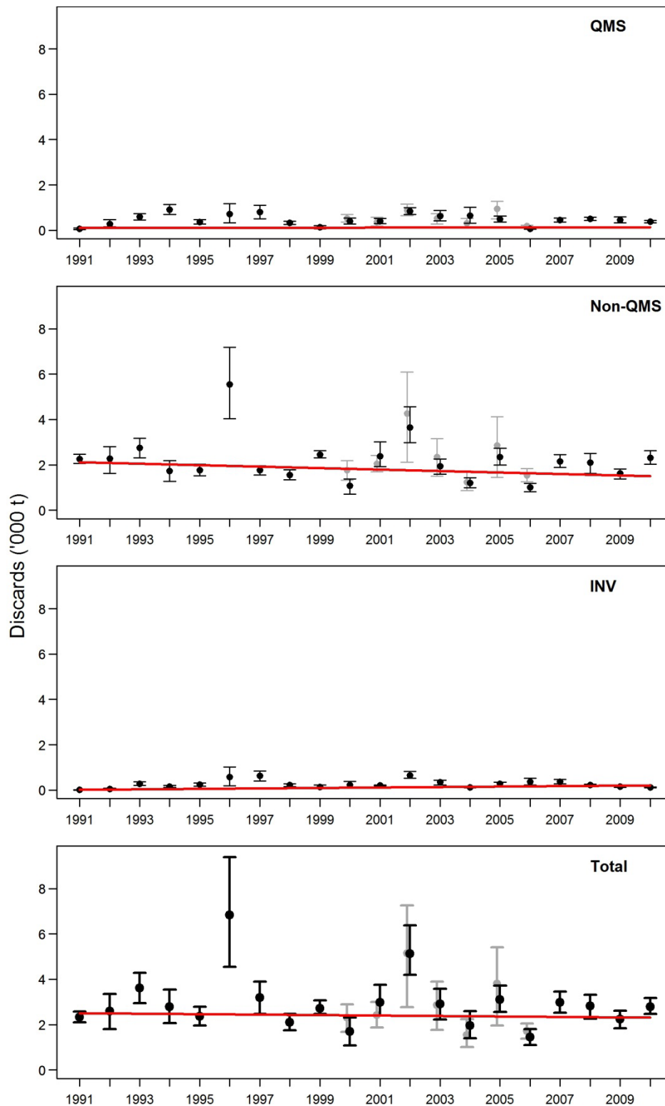
Figure 6.19: Annual estimates of discards in the scampi trawl fishery, for QMS species, non-QMS species, invertebrates (INV), and overall for 1990–91 to 2009–10. Also shown (in grey) are estimates of discards in each category (excluding INV) calculated for 1999–2000 to 2005–06 (Ballara & Anderson 2009). Error bars indicate 95% confidence intervals. The straight lines show the fit of the weighted regression to annual discards.
