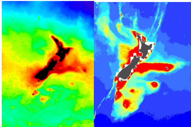
Figure 8.4: Left panel: Ocean colour in the New Zealand region from satellite imagery. Red shows the highest intensity of ocean colour typically associated with higher primary productivity. Right panel: The relative concentrations of particulate organic carbon (POC) that reach the seafloor. Red shows the highest levels, which are likely to be associated with areas of enhanced benthic productivity (based on the model of Lutz et al. (2007)). Images courtesy of NIWA.
