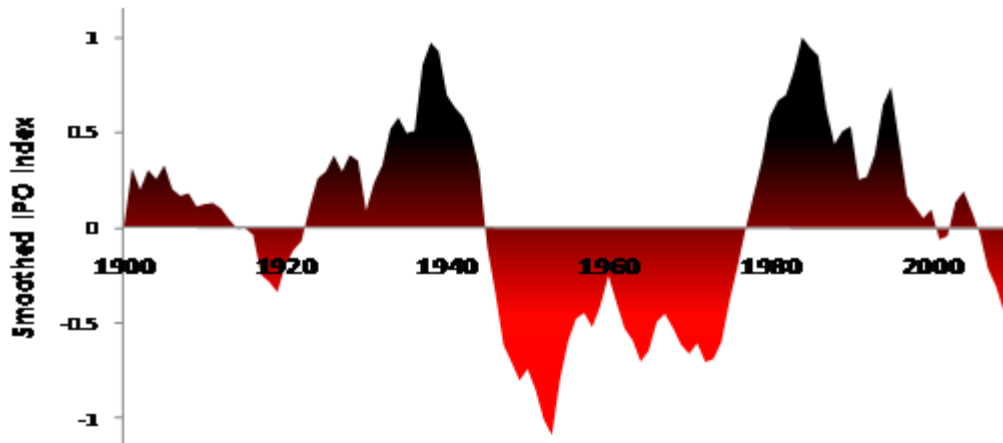
Figure 8.11: Smoothed index of the Interdecadal Pacific Oscillation (IPO) since 1900. (Image source NIWA based on data from the United Kingdom Meteorological Office, UKMO).
