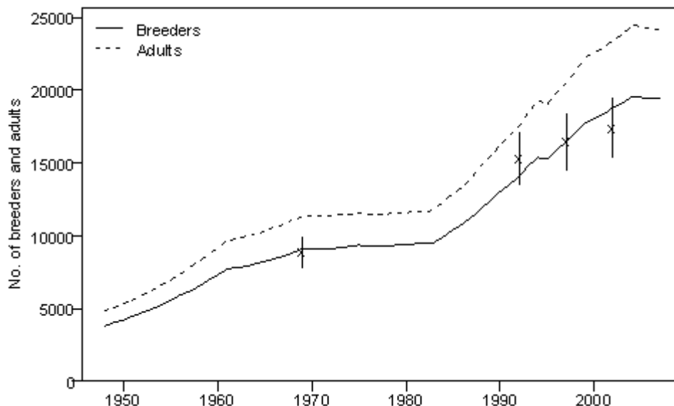
Figure 5.17 (reproduced from Francis et al. 2008): Estimates from model SBA21 of numbers of breeders (solid line) and adults (broken line) in each year. Also shown are the census observations (after (Sagar and Stahl 2005) of numbers of breeders (crosses), with assumed 95% confidence intervals (vertical lines).
