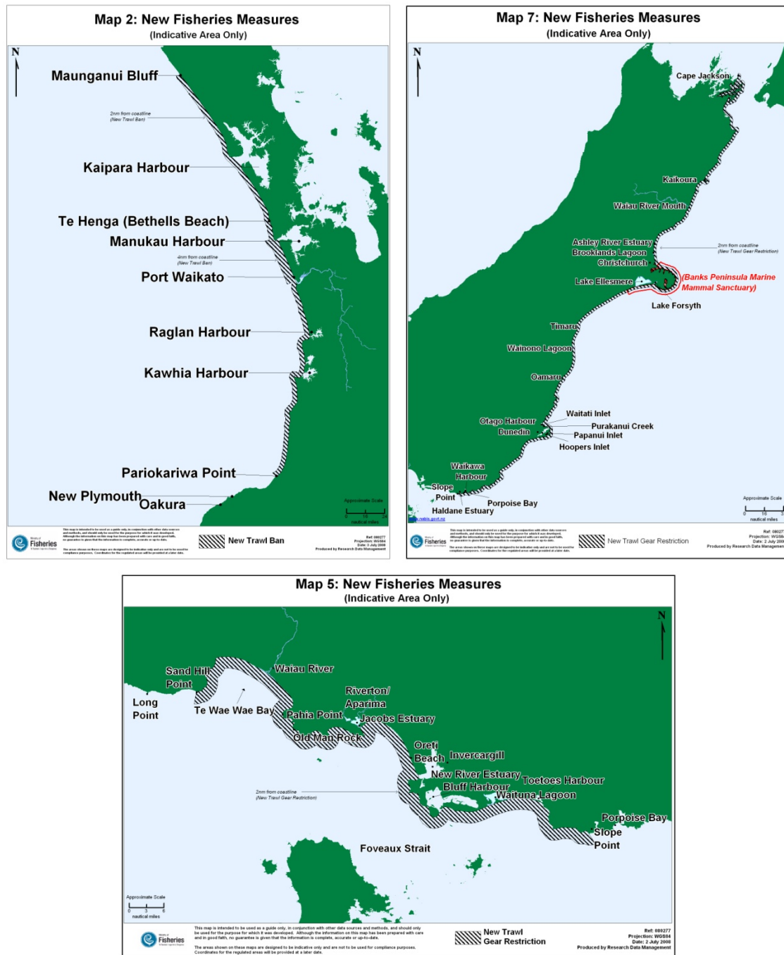
Figure 7.2: Maps from Ministry of Fisheries website showing the general locations of areas closed to trawling to protect Hector's and Maui's dolphins. Note scales differ. ( http://www.fish.govt.nz/en/nz/Consultations/Archive/2008/Hectors+dolphins/Decisions.htm?wbc_purpose=Basic&WBCMODE=PresentationUnpublished%2525252525252cPresentationUnpublished )
