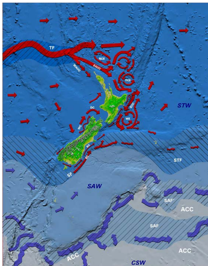
Figure 8.5: Circulation around New Zealand. TF Tasman Front (large red arrows), WAUC West Auckland Current, EAUC East Auckland Current, NCE North Cape Eddy, ECE East Cape Eddy, ECC East Cape Current, WE Wairarapa Eddy, DC D'Urville Current, WC Westland Current, SC Southland Current, SF Southland Front, STW Subtropical Water, STF Subtropical Front (left diagonal hashed area), SAW Subantarctic Water, SAF Subantarctic Front (right diagonal hashed area), ACC Antarctic Circumpolar Current, CSW Circumpolar Surface Water, DWBC Deep Western Boundary Current (large purple arrows) (after Carter et al. 1998).
