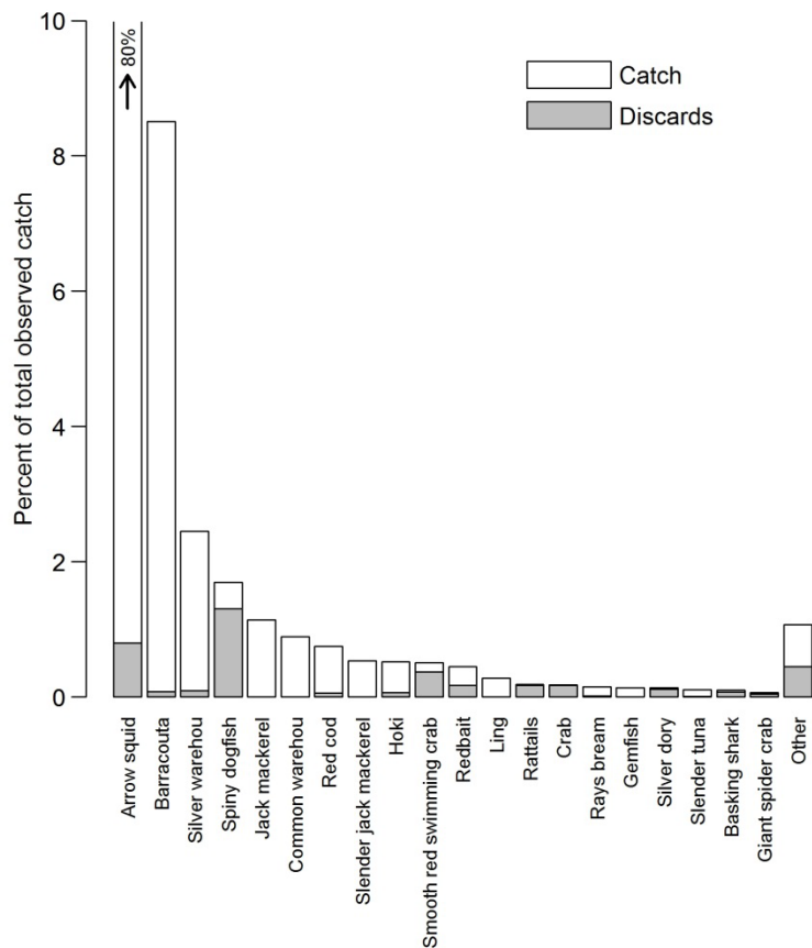
Figure 6.1: Percentage of the total catch contributed by the main bycatch species (those representing 0.05% or more of the total catch) in the observed portion of the arrow squid fishery, and the percentage discarded. The “Other” category is the sum of all bycatch species representing less than 0.05% of the total catch.
