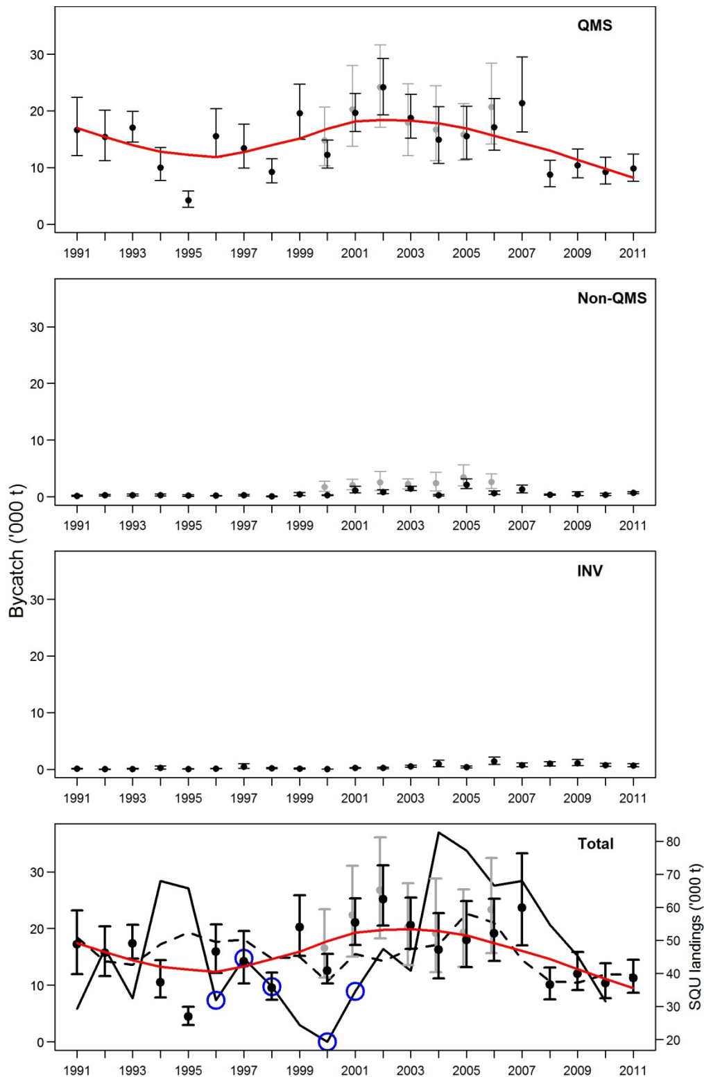
Figure 6.2: Annual estimates of bycatch in the arrow squid trawl fishery, for QMS species, non-QMS species, invertebrates (INV), and overall for 1990–91 to 2010–11. Also shown (in grey) are estimates of bycatch in each category (excluding INV) calculated for 1999–2000 to 2005–06 (Ballara & Anderson 2009). Error bars indicate 95% confidence intervals. The red lines show the fit of a locally-weighted polynomial regression to annual bycatch. In the bottom panel the solid black line shows the total annual reported trawl-caught landings of arrow squid (Ministry of Fisheries 2011), with circles indicating years in which the fishery closed early after reaching the sea lion FRML; and the dashed line shows annual effort (scaled to have mean equal to that of total bycatch).
