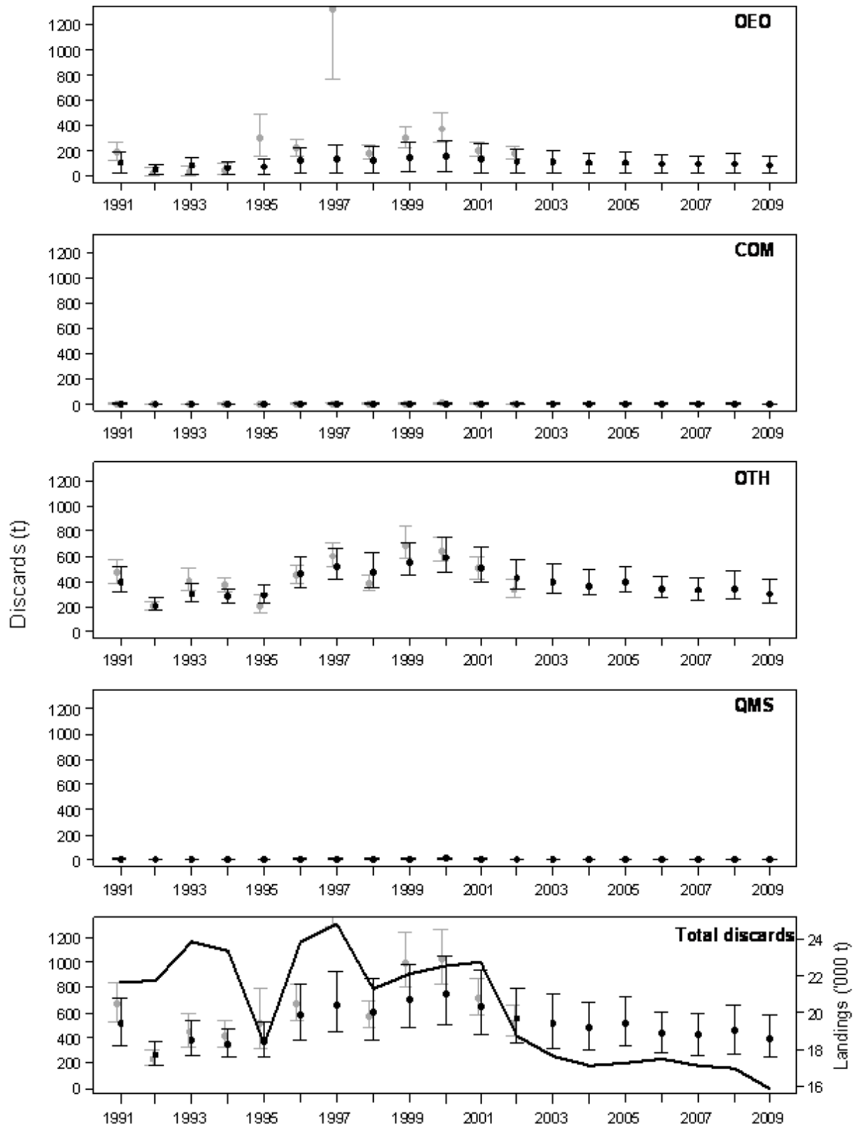
Figure 6.16: Annual estimates of fish discards in the oreo trawl fishery, calculated for the target species (OEO), commercial species (COM), non-commercial species (OTH), QMS species, and overall for 1990–91 to 2008–09 (black points). Also shown (grey points) are estimates of discards in each category (excluding QMS) calculated for 1990–91 to 2001–02 (Anderson 2004a). Error bars show the 95% confidence intervals. The black line in the bottom panel shows the total annual estimated landings of oreos (Ministry of Fisheries 2010).
