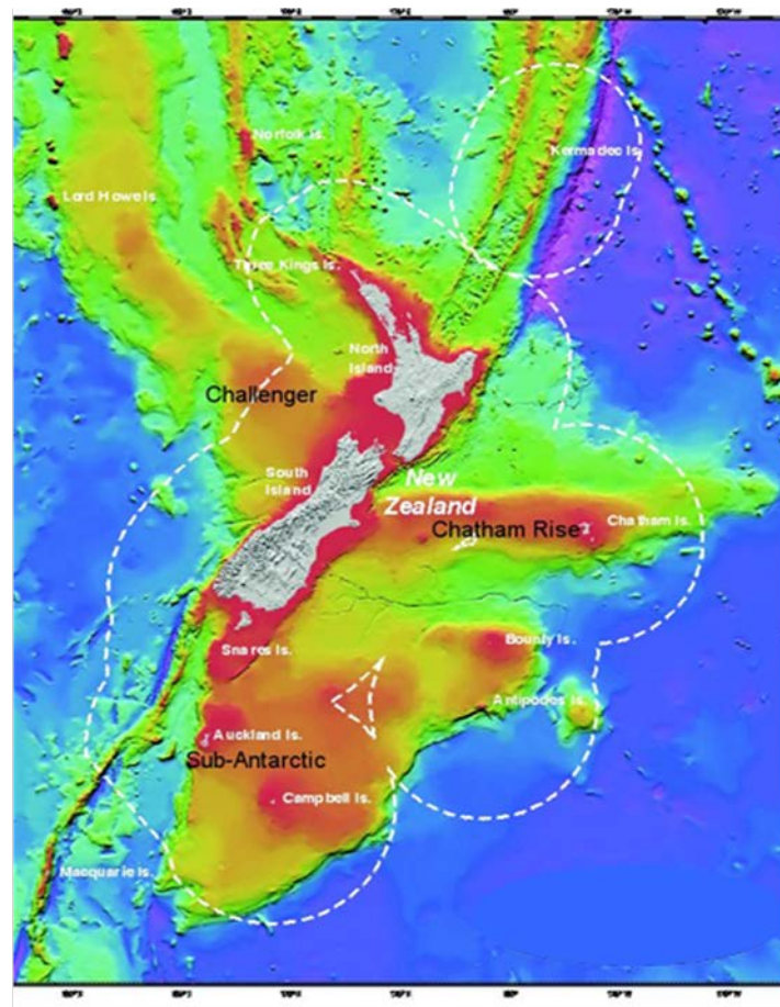
Figure 8.2 Undersea topography of New Zealand (red shallow to blue deep). White dash line shows the EEZ boundary. Image courtesy of NIWA.
