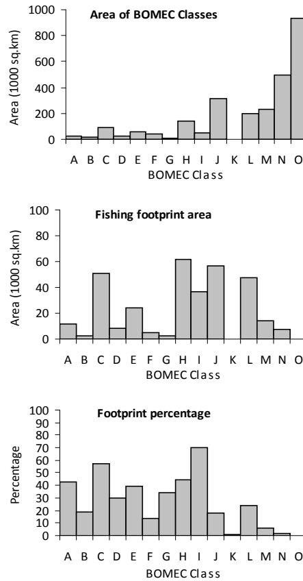
Figure 7.12: Plots from Baird and Wood (2010) of the areas of each BOMECE Class (top), the fishing footprint up to 2004/05 shown in Figure 7.8 (centre), and percentage of each BOMECE Class area covered by the fishing footprint (bottom).
