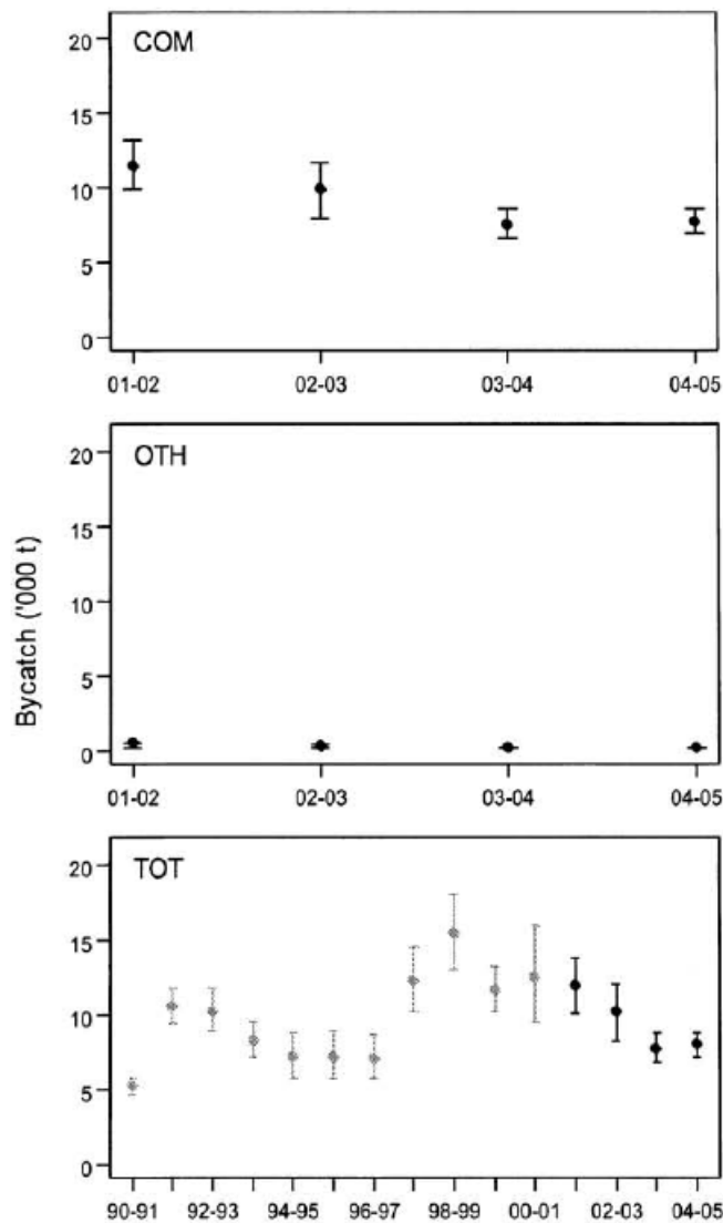
Figure 6.9: Annual estimates of fish bycatch in the target jack mackerel trawl fishery for the 2001-02 to 2004-05 fishing years (in black), calculated for commercial species (COM), non-commercial species (OTH), and overall (TOT). Also shown (in grey) are estimates of overall bycatch calculated for 1990-91 to 2000-01 by Anderson et al. (2000) and Anderson (2004a). Error bars show the 95% confidence intervals.
