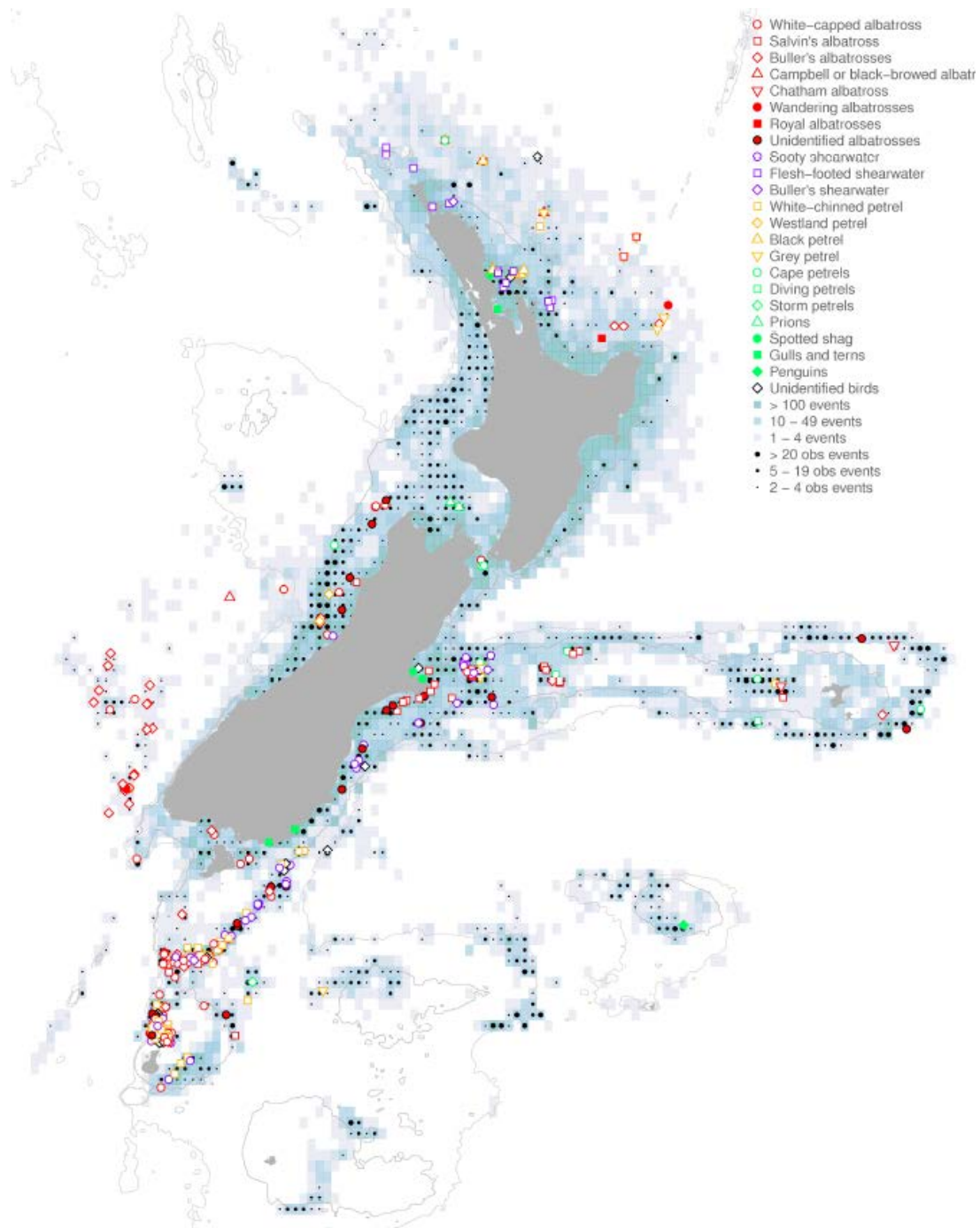
Figure 5.3 (reproduced from Abraham and Thompson 2011): All observed seabird captures in trawl, surface longline, and bottom longline fishing within the New Zealand region, between October 2008 and September 2009. The colour within each 0.2 degree cell indicates the number of fishing events (tows and sets, darker colours indicate more fishing) and the black dots indicate the number of observed events (larger dots indicate more observations). The coloured symbols indicate the location of observed seabird captures, randomly jittered by 0.2 degrees. The 500 m and 1000 m depth contours are shown.
