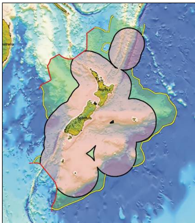
Figure 8.1: New Zealand land mass area 250,000 km 2 ; EEZ & territorial sea area (pink) 4,200,000 km 2 ; extended continental shelf extension area (light green) 1,700,000 km 2 ; Total area of marine jurisdiction 5,900,000 km 2 . The black line shows the boundary of the New Zealand EEZ, the yellow line indicates the extension to New Zealand's legal continental shelf, and the red line the agreed Australia/New Zealand boundary under UNCLOS Article 76. Image courtesy of GNS.
