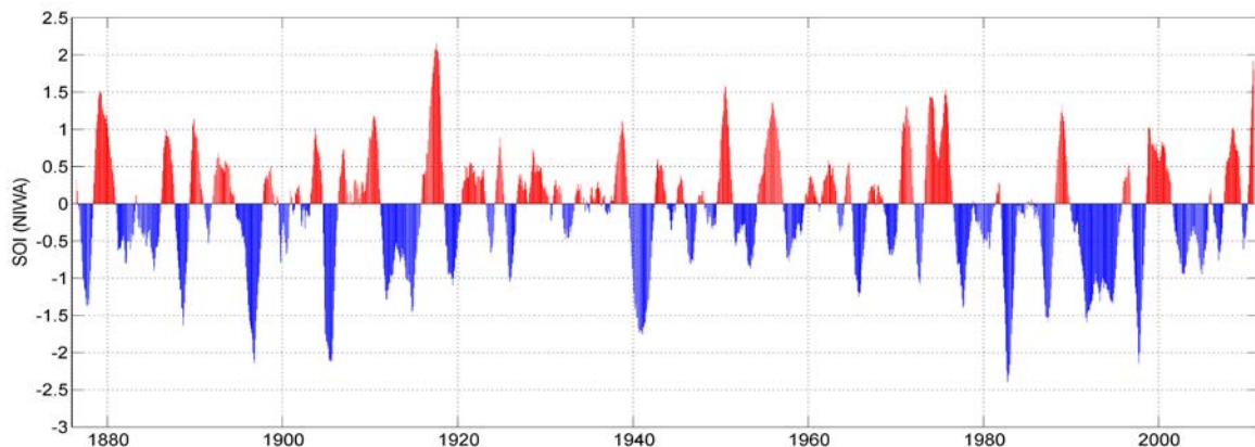
Figure 8.12: Southern Oscillation Index (SOI) 13-month running mean 1876-2010. Red indicates warmer temperatures, blue indicates cooler conditions for New Zealand. (Image courtesy of NIWA.)
