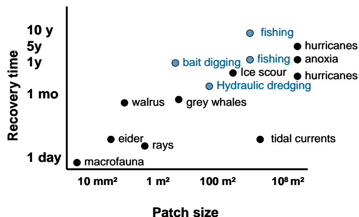
Figure 7.4: General relation between the spatial extent of disturbance events and the time taken to recover from such events in marine systems (after Kaiser et al. 2003). Blue dots signal human impacts, including fishing in habitats of different abilities to recover, and black dots signal natural disturbance.
