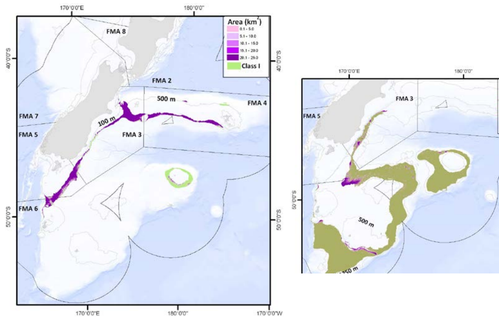
Figure 7.13: Maps from Baird and Wood (2010) showing BOMECEC classes I (left) and M (right) overlaid with the footprint of trawls on or near the seafloor reported on TCEPR forms to 2004–05 for each 25-km 2 cell.
