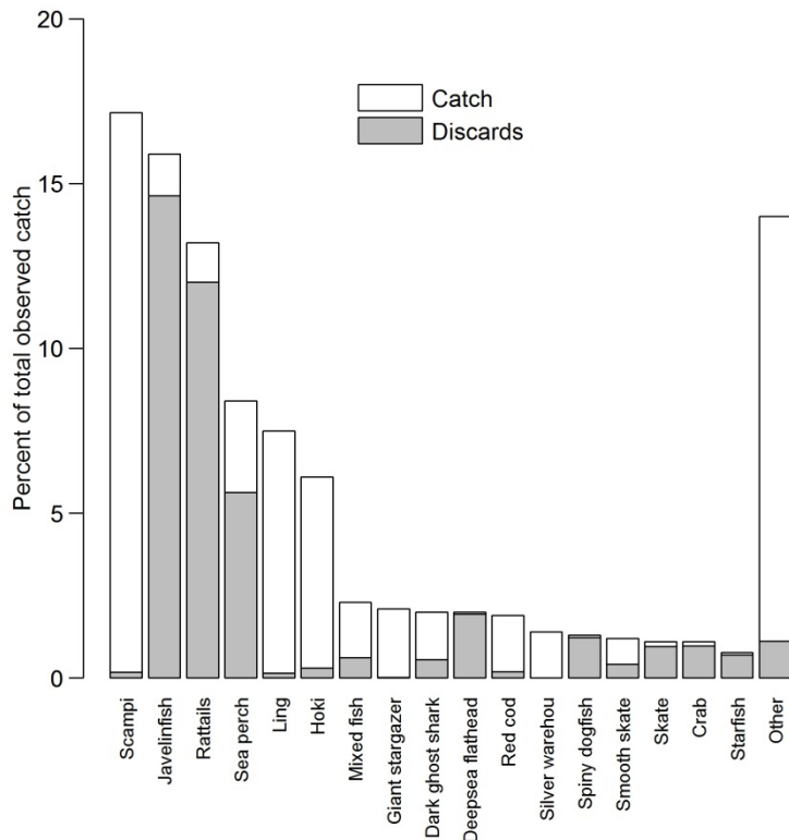
Figure 6.17: Percentage of the total catch contributed by the main bycatch species (those representing 1% or more of the total catch) in the observed portion of the scampi fishery, and the percentage discarded. The “Other” category is the sum of all other bycatch species (fish and invertebrates) representing less than 1% of the total catch.
