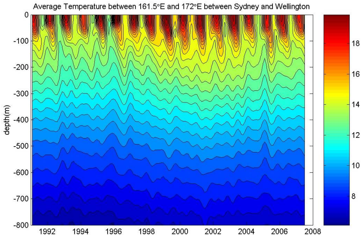
Figure 8.10: Eastern Tasman ocean temperature: Wellington to Sydney 1991–2008. Coloured scale to the right is temperature °C. (Image from Hurst et al. 2012, after Sutton et al. 2005)
