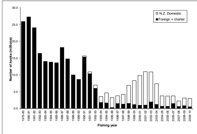
Figure 6.20: Effort (hooks set) in the tuna longline fishery. Black bars are Foreign and Charter vessels, white bars are NZ domestic vessels.
