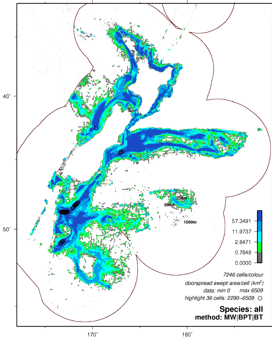
Figure 7.7: Map from Baird et al. 2011 showing the intensity of bottom-contacting trawling effort reported on TCEPR forms 1989–90 to 2004–05. The colour scale indicates the aggregate swept area estimated by Baird et al. for each 5 x 5 km cell, all target species combined (e.g., the 36 most intensively fished 25 km 2 cells all had an aggregate swept area of over 2290 km 2 over 16 years, which translates to the seabed in those cells being swept by some part of a trawl 92 times in 16 years, or an average of 5.8 or more times each year). Updates for deepwater trawl fisheries are expected in 2013.
