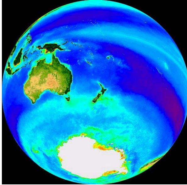
Figure 8.3: SeaWiFS image showing elevated chlorophyll a (green) near New Zealand. Image courtesy of NOAA
