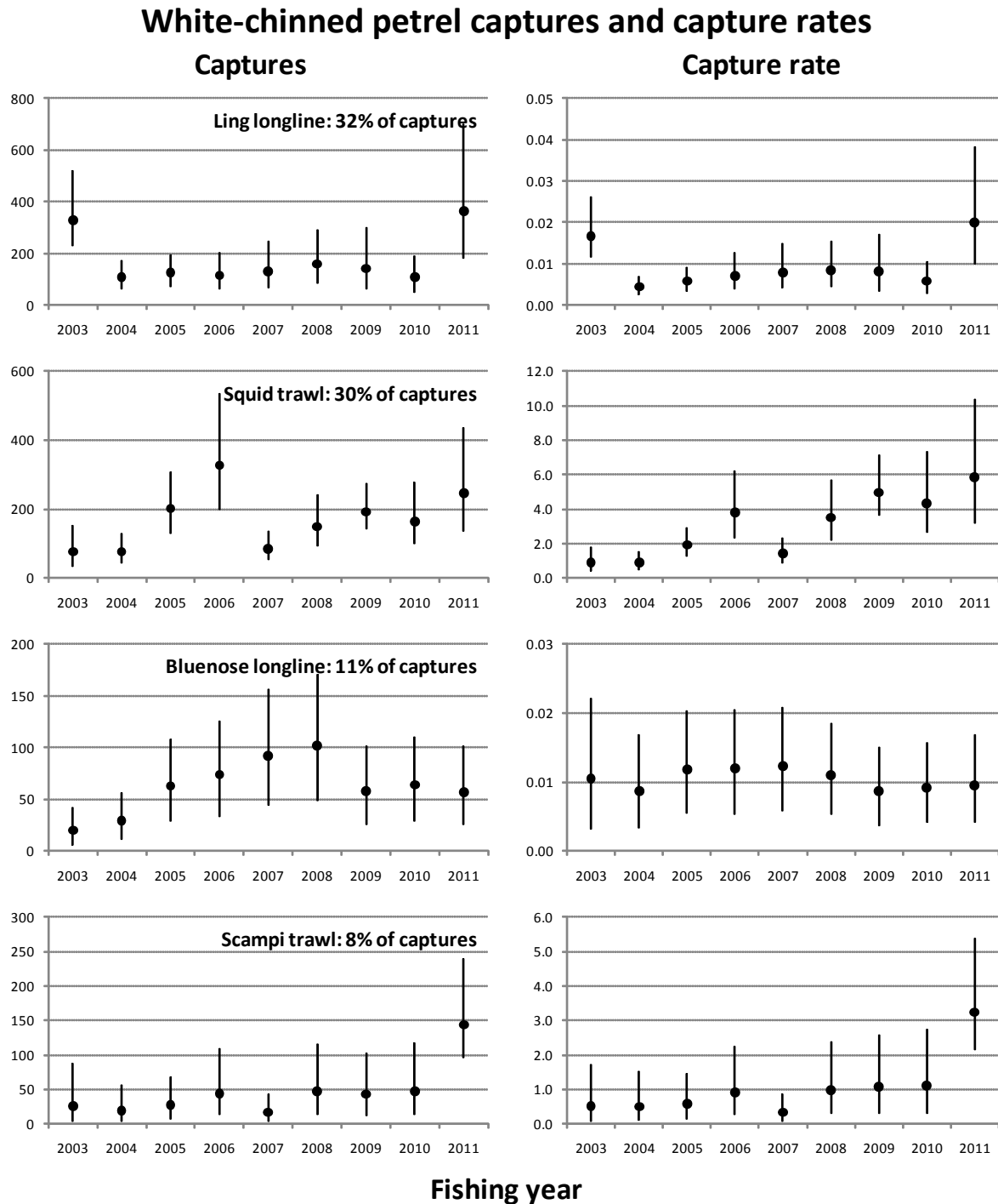
Figure 5.9: Model-based estimates of captures (left panels) and capture rates (right panels, captures per 100 trawl tows or 1000 longline hooks) of white chinned petrels in the four fisheries estimated to have taken the most captures between 2002/03 and 2010/11 (cumulatively, 81% of all white-chinned petrel captures). Data version v20121101.
