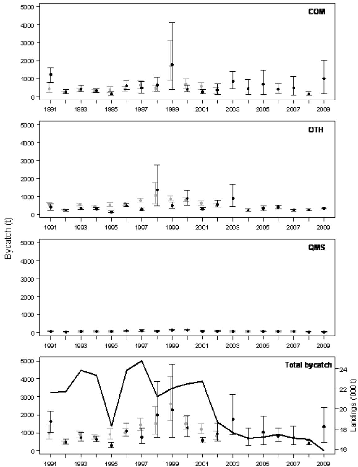
Figure 6.15: Annual estimates of fish bycatch in the oreo trawl fishery, calculated for commercial species (COM), non-commercial species (OTH), QMS species, and overall for 1990-91 to 2008-09 (black points). Also shown (grey points) are estimates of bycatch in each category (excluding QMS) calculated for 1990-91 to 2001-02 (Anderson 2004a). Error bars show the 95% confidence intervals. The black line in the bottom panel shows the total annual estimated landings of oreos (Ministry of Fisheries 2010).
