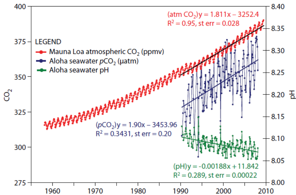
Figure 8.15: Time series of atmospheric carbon dioxide at Moana Loa, seawater carbon dioxide and surface ocean pH at Ocean station ALOHA in the subtropical North Pacific Ocean near Hawaii. pH is shown as in situ pH, based on direct measurements and calculated from dissolved inorganic carbon and alkalinity in the surface layer (after Dore et al. 2009). (Image directly sourced from Feely et al. 2009 with permission.)
