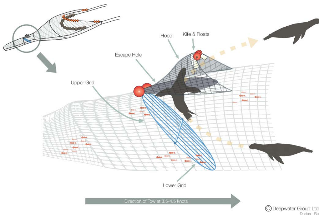
Figure 3.2: Diagram of a NZ sea lion exclusion device (SLED) inside a trawl net. Image courtesy of the Deepwater Group.
