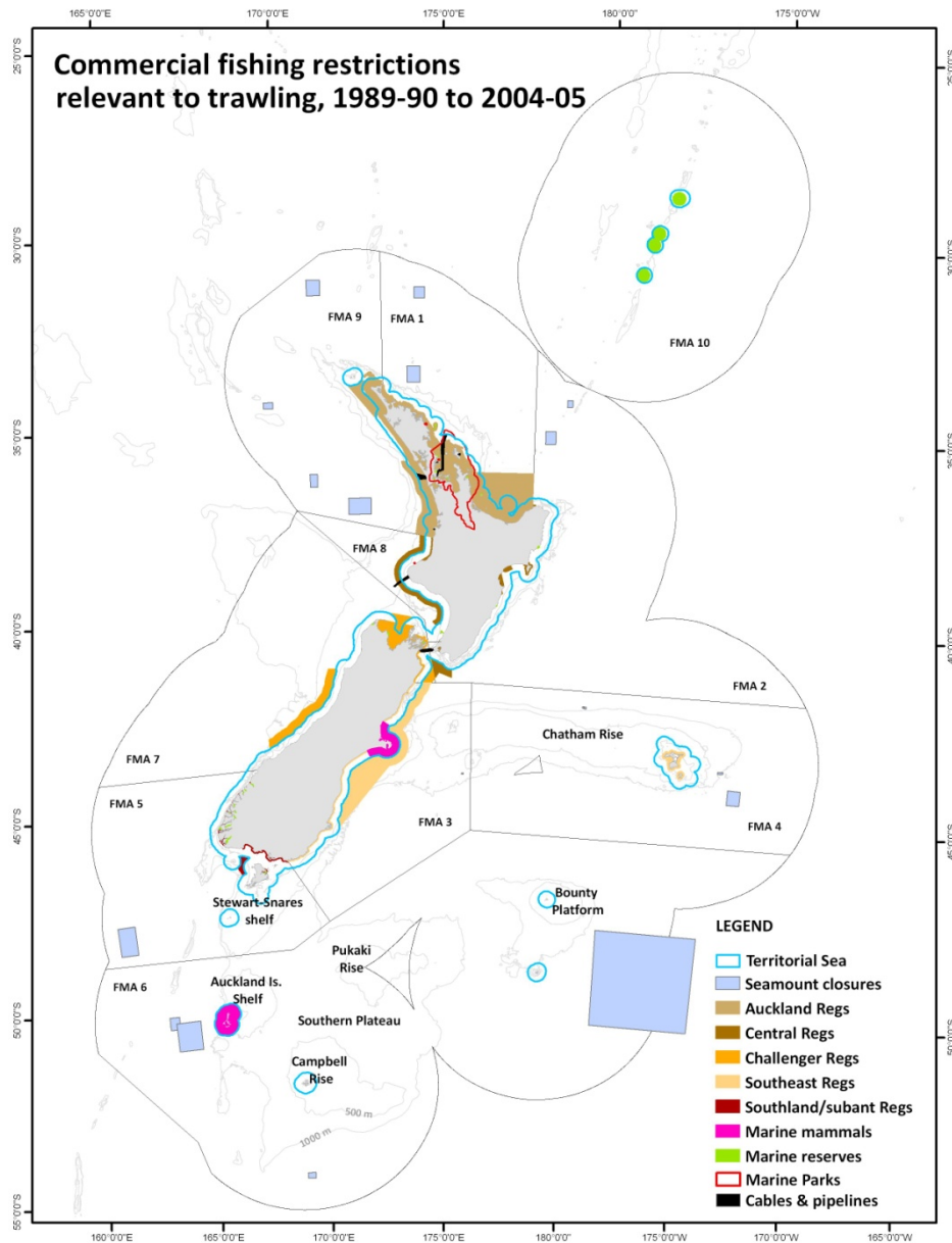
Figure 7.1: Map, from Baird and Wood 2010, of the major spatial restrictions to trawling present at some stage during 1989–90 to 2004–05 and the Ministry for Primary Industries Fishery Management Areas (FMAs) within the outer boundary of the New Zealand EEZ. Vessels longer than 28 m may not trawl within the TS and additional restrictions are specified in the Fisheries (Auckland Kermadecs Commercial Fishing) Regulations 1986, the Fisheries (Central Area Commercial Fishing) Regulations 1986, the Fisheries (Challenger Area Commercial Fishing) Regulations 1986 the Fisheries (South East Area Commercial Fishing) Regulations 1986, and the Fisheries (Southland and Sub-Antarctic Areas Commercial Fishing) Regulations 1991.
