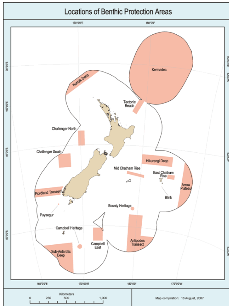
Figure 7.3: Map from Ministry of Fisheries website showing the general locations of Benthic Protection Areas (BPAs) ( http://www.fish.govt.nz/en-nz/Environmental/Seabed+Protection+and+Research/Benthic+Protection+Areas.htm?wbc_purpose=basic&WBCMODE=presentationunpublished&MSHiC=65001&L=10&W=BPA%20&Pre=%3Cspan%20class%3d'SearchHighlight'%3E&Post=%3C/span%3E ). See also Helson et al. 2009.
