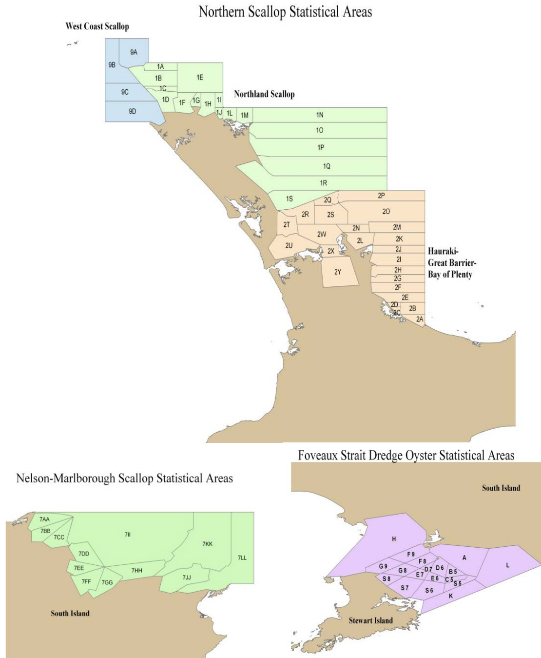
Figure 7.10: Maps taken from Baird et al. 2011 of statistical reporting areas for the main oyster and scallop dredge fisheries (scales differ). Note that these reporting areas are generally much smaller than the standard statistical reporting areas used for most finfish reporting.
