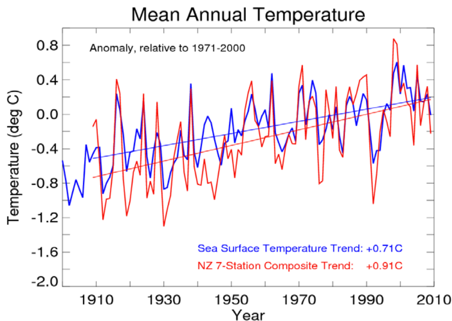
Figure 8.6: Annual time series in New Zealand. NOAA annual mean sea surface temperatures (blue line) 25 and NIWA's seven-station annual mean air temperature composite series (red line), expressed as anomalies relative to the 1971-2000 climatological average. Linear trends over the period 1909-2009, in °C/century, are noted under the graph. (Image Source Mullan et al. 2010)
