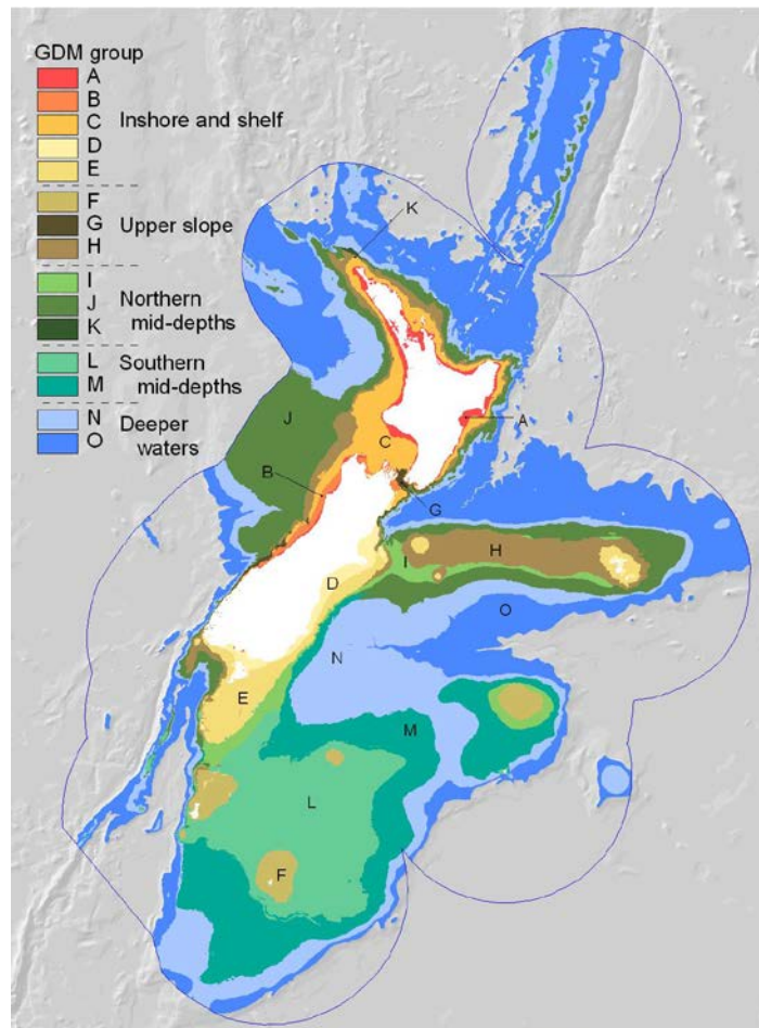
Figure 7.6: Map of the distribution of Benthic Optimised Marine Environment Classification (BOME) classes defined by multivariate classification of environmental data transformed using results from GDM analyses of relationships between environment and species turnover averaged across eight taxonomic groups of benthic species. From Leathwick et al. 2010.
