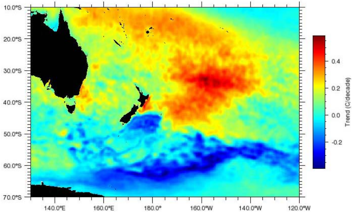
Figure 8.8: Trends in sea surface temperature, in ^{\circ}\text{C}/\text{decade} over the period 1982-2009. The data are again taken from NOAA, but are based on daily interpolated satellite measurements over a much finer 0.25^{\circ} grid. See http://www.ncdc.noaa.gov/oa/climate/research/sst/oi-daily.php . This product is the result of an objective analysis, an optimum interpolation rather than a pure satellite retrieval, so as to correct for issues like the effect of the Mt Pinatubo eruption aerosols on satellite detected radiances. It is described in Reynolds et al. (2007)
