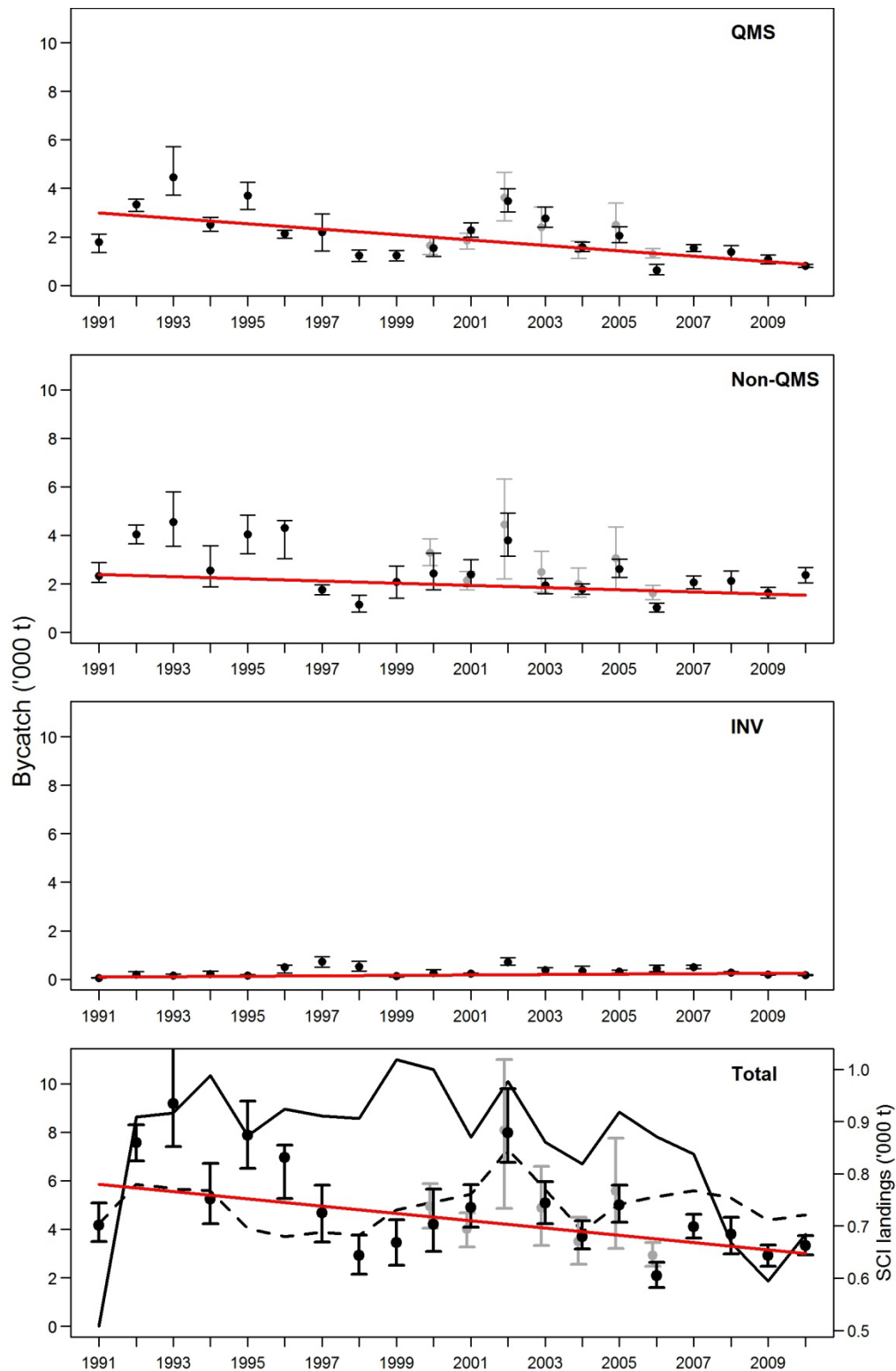
Figure 6.18: Annual estimates of bycatch in the scampi trawl fishery, for QMS species, non-QMS species, invertebrates (INV), and overall for 1990–91 to 2009–10. Also shown (in grey) are estimates of bycatch in each category (excluding INV) calculated for 1999–2000 to 2005–06 (Ballara & Anderson 2009). Error bars indicate 95% confidence intervals. The straight lines show the fit of a weighted regression to annual bycatch. In the bottom panel the solid black line shows the total annual reported landings of scampi (Ministry of Fisheries 2011) and the dashed line shows annual effort (scaled to have mean equal to that of total bycatch).
