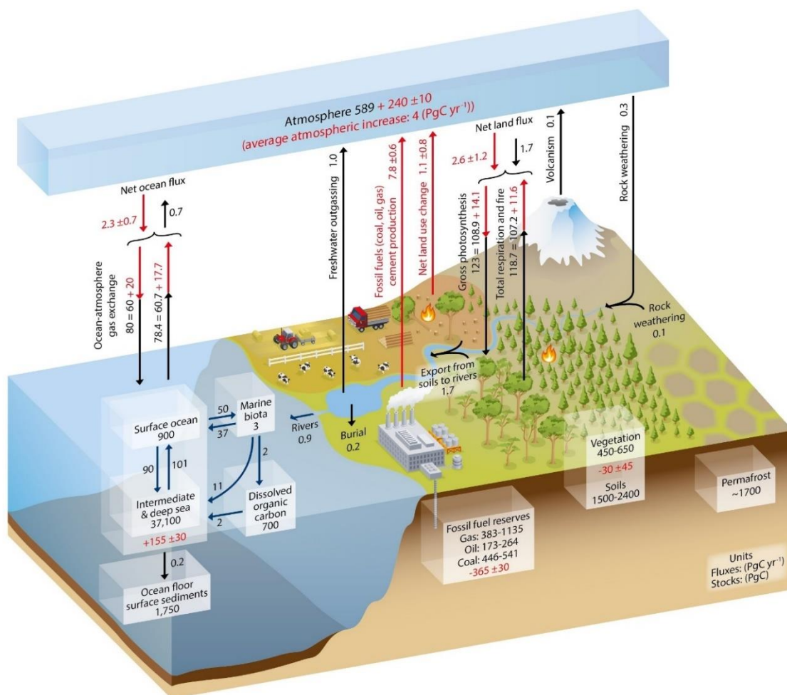
Figure 6-1: Simplified schematic of the global carbon cycle (IPCC, 2013)
