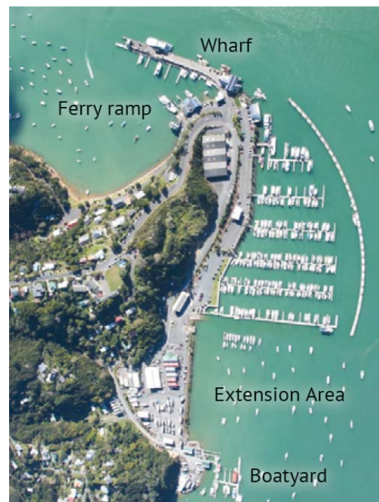
Figure 41. Opua marina proposed expansion
