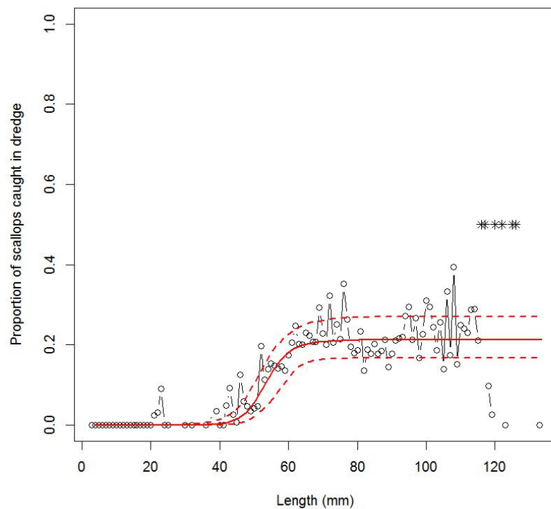
Figure 2: SCA 7 ring-bag dredge efficiency (from Tuck et al. 2018). The plotted curve is a logistic capped selectivity ogive ( L_{50} = 53.3\text{mm} , a_{95} = 7.3\text{mm} , a_{\text{max}} = 0.21 ) fitted to the proportion of scallops retained in the dredge. Solid line is the fit to all data in the 2018 study and dashed lines represent 95% CI of selectivity at each length.
